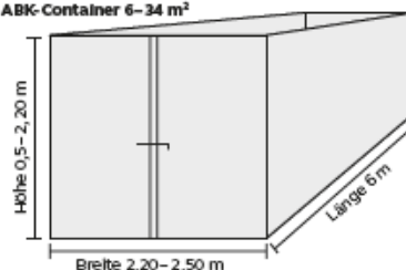
ABK-Container 6–34 m 3
